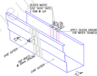
EAVE GUTTER LAP DETAIL (TYP.)
