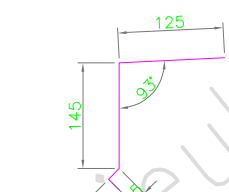
EAVE FLASHING PROFILE
