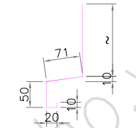
DRIP TRIM PROFILE
