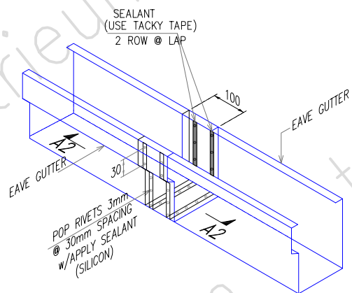
EAVE GUTTER LAP DETAIL (TYP.)
