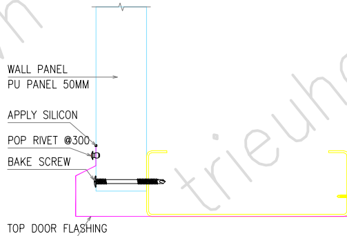
DETAIL TOP ROLL UP DOOR AND SINGLE DOOR FLASHING
