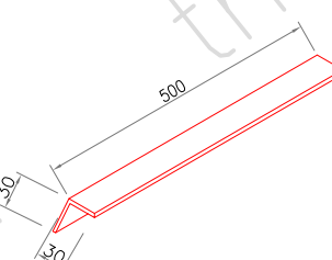
GUTTER SUPPORT L30x30x2 (GALVANIZE)
