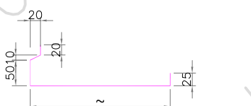
TOP DOUBLE DOOR FLASHING PROFILE
