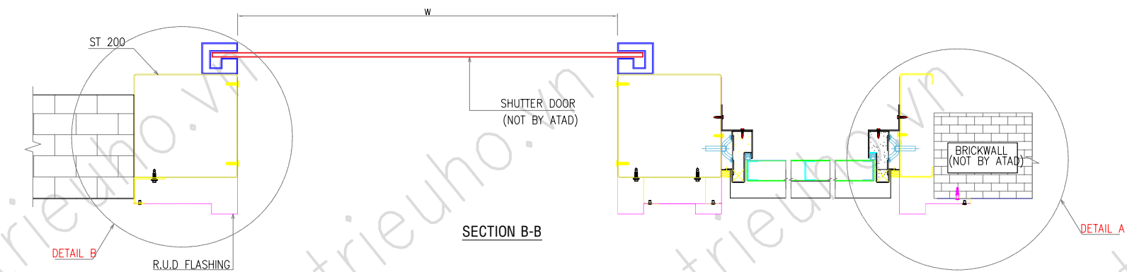
TOP ROLL UP DOOR AND SINGLE DOOR FLASHING PROFILE
