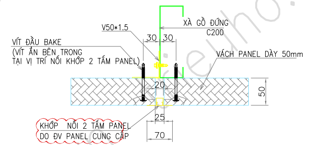
DETAIL CONECTION TOLE PU PANEL 50MM
