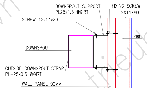
CONNECT DOWNSPOUT TO GIRT DETAIL (TYP.)
