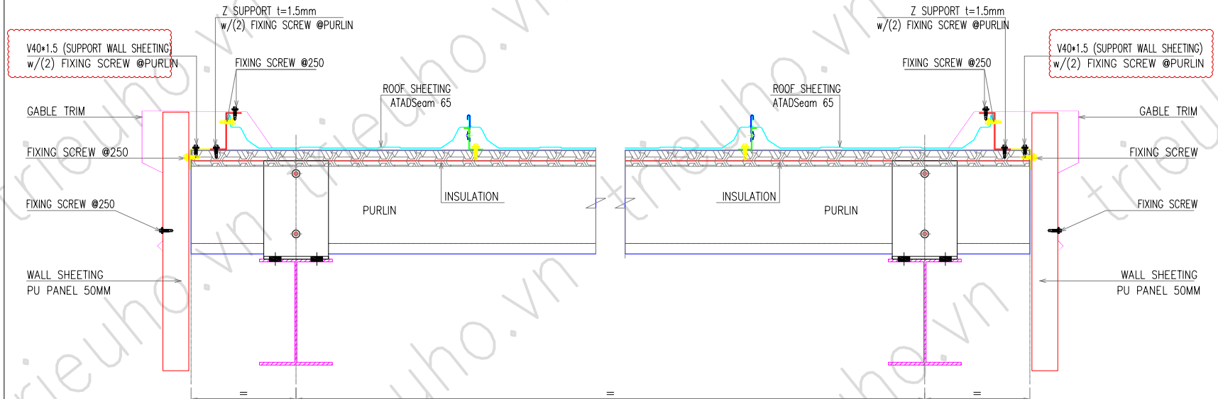
GABLE TRIM DETAIL (TYP.)
