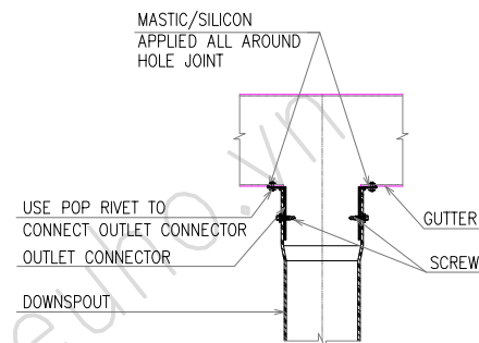
CONNECT DOWNSPOUT TO GUTTER DETAIL (TYP.)
