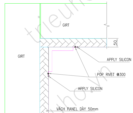
DETAIL CORNOR TRIM
