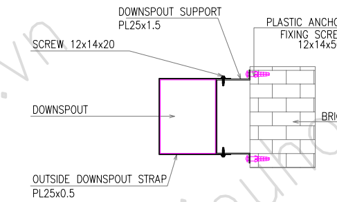
CONNECT DOWNSPOUT TO BRICKWALL DETAIL (TYP.)
