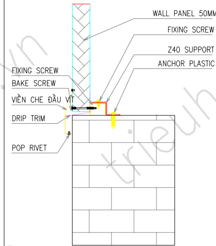
DRIP TRIM DETAIL (TYP.)
