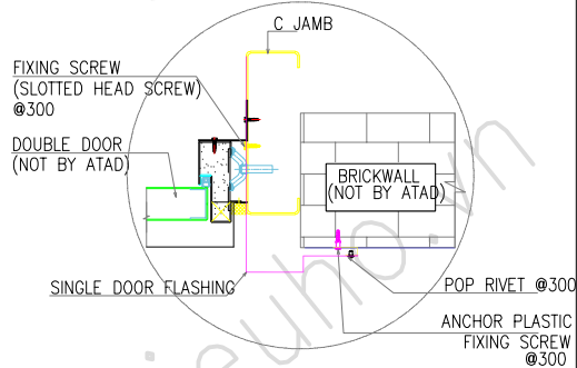
DETAIL A PROFILE
