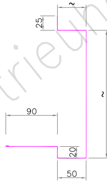
BESIDE SINGLE DOOR FLASHING PROFILE
