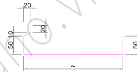
TOP ROLL UP DOOR AND SINGLE DOOR FLASHING PROFILE
