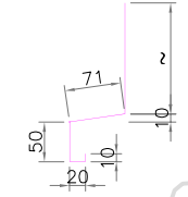
DRIP TRIM PROFILE
