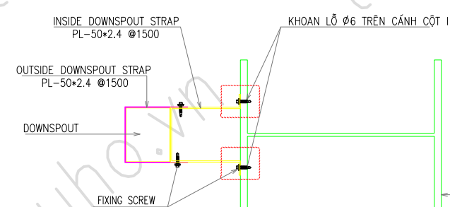
CONNECT DOWNSPOUT TO COLUMN DETAIL (TYP.)
