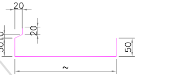
TOP SINGLE DOOR FLASHING PROFILE
