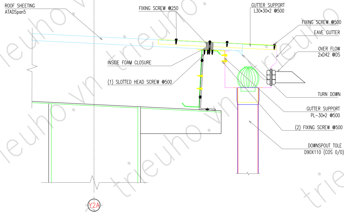
EAVE GUTTER DETAIL (TYP.) @G.L Y2A FRAMING @G.L X16 TO @G.L X17
