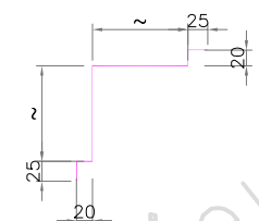
CORNOR TRIM FLASHING
