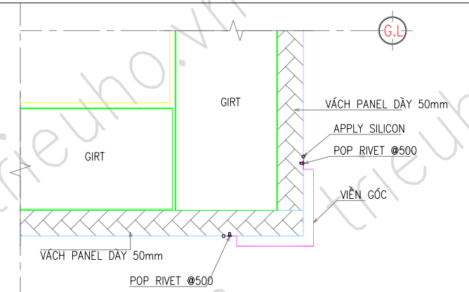
DETAIL CORNOR TRIM
