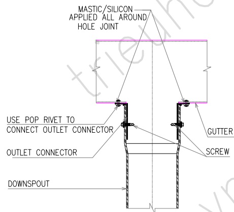
CONNECT DOWNSPOUT TO GUTTER DETAIL (TYP.)
