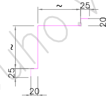
CORNOR TRIM FLASHING
