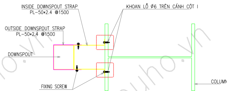
CONNECT DOWNSPOUT TO COLUMN DETAIL (TYP.)
