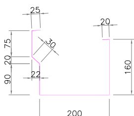
EAVE GUTTER PROFILE
