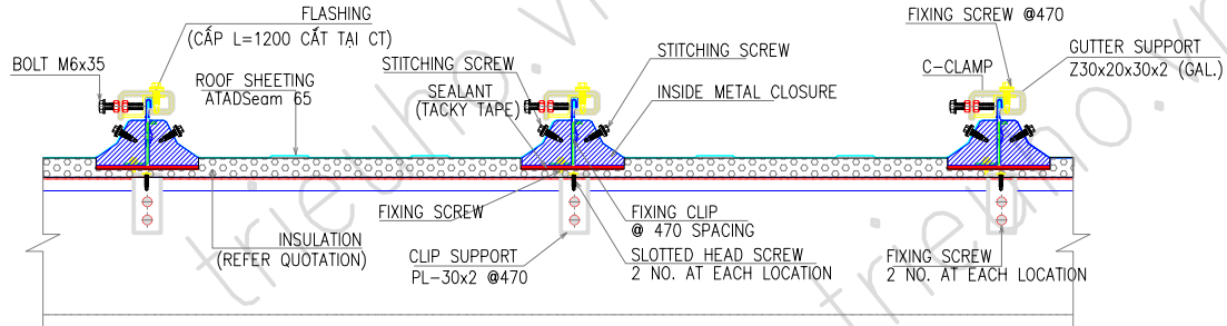
SECTION A1-A1
