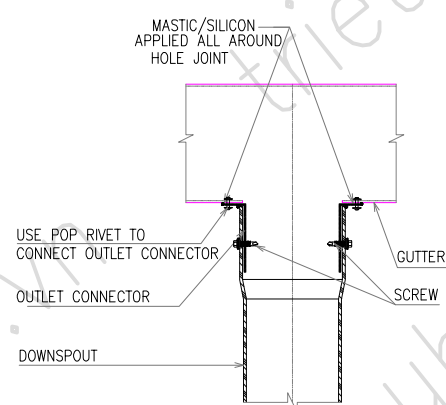
CONNECT DOWNSPOUT TO GUTTER DETAIL (TYP.)
