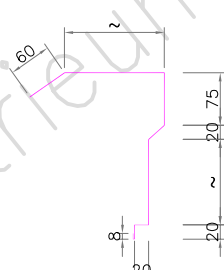
GABLE TRIM DETAIL (TYP.)
