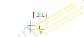
GUTTER SUPPORT t=2.0mm DETAIL (TYP.) (@470)
