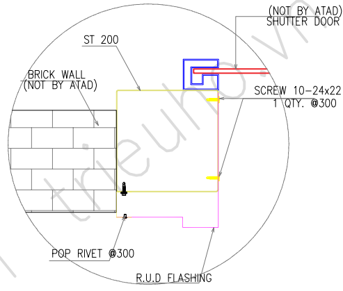
DETAIL B PROFILE
