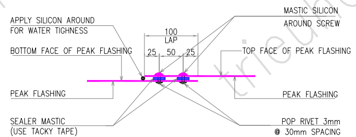
SECTION A1-A1
