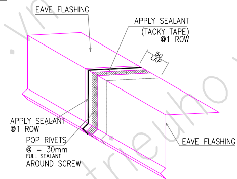
EAVE FLASHING LAP DETAIL (TYP.)
