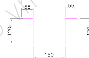
VALLEY GUTTER PROFILE
