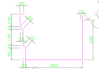
EAVE GUTTER PROFILE ( STAINLESS STEEL)
