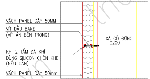
DETAIL CONECTION TOLE PU PANEL 50MM
