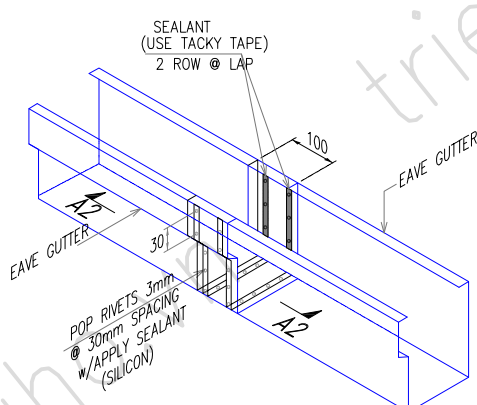
EAVE GUTTER LAP DETAIL (TYP.)
