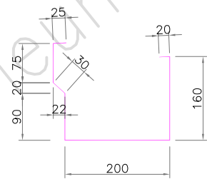
EAVE GUTTER PROFILE
