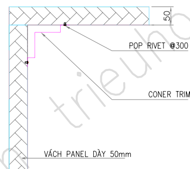
DETAIL CORNOR TRIM
