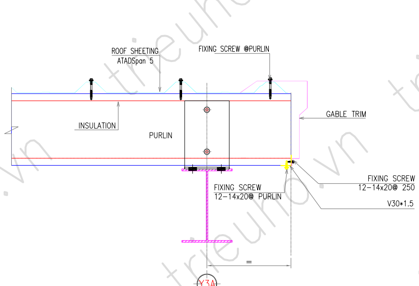
GABLE TRIM DETAIL (TYP.)
