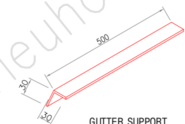
GUTTER SUPPORT L30x30x2 (GALVANIZE)
