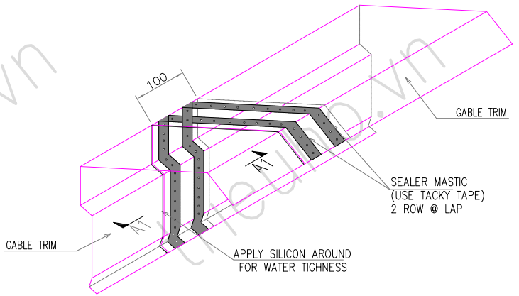
GABLE TRIM LAP DETAIL (TYP.)
