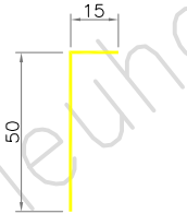
PEAK FLASHING PROFILE
