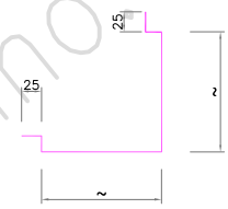
CORNOR TRIM FLASHING
